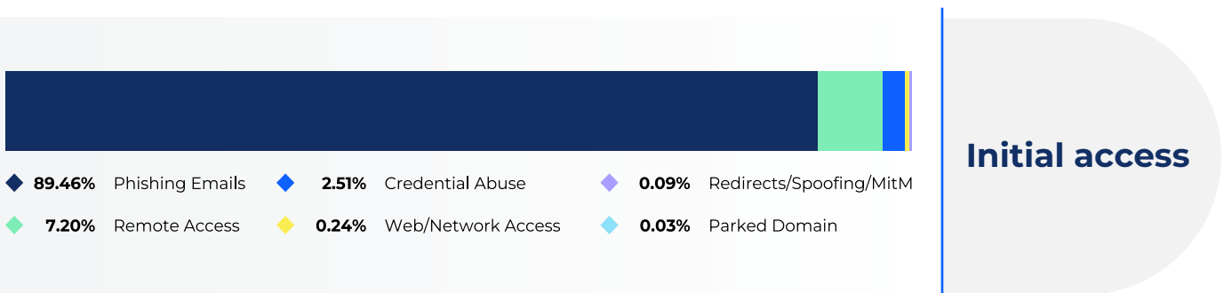
Figure 2: Tactics used to gain initial access to networks and systems
