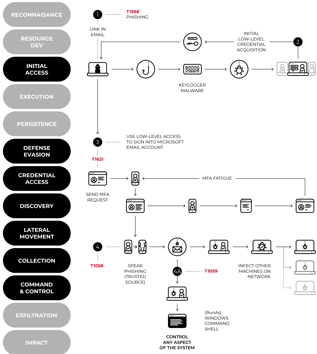
Figure 4: The MITRE ATT&CK® Framework highlights the importance of implementing a comprehensive set of controls to defend yourself holistically across application, identity, network, and server resources. In this example, identified by our Security Operations Center (SOC), a single user clicking on a phishing email started a chain of events that ended with the adversary gaining access to the Windows PowerShell Command Line Interface (CLI).
